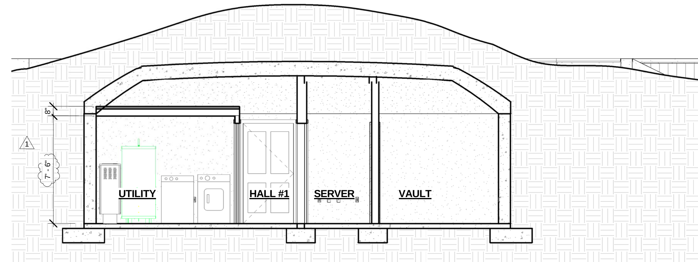
① SECTION 3 1/4" = 1'-0"
