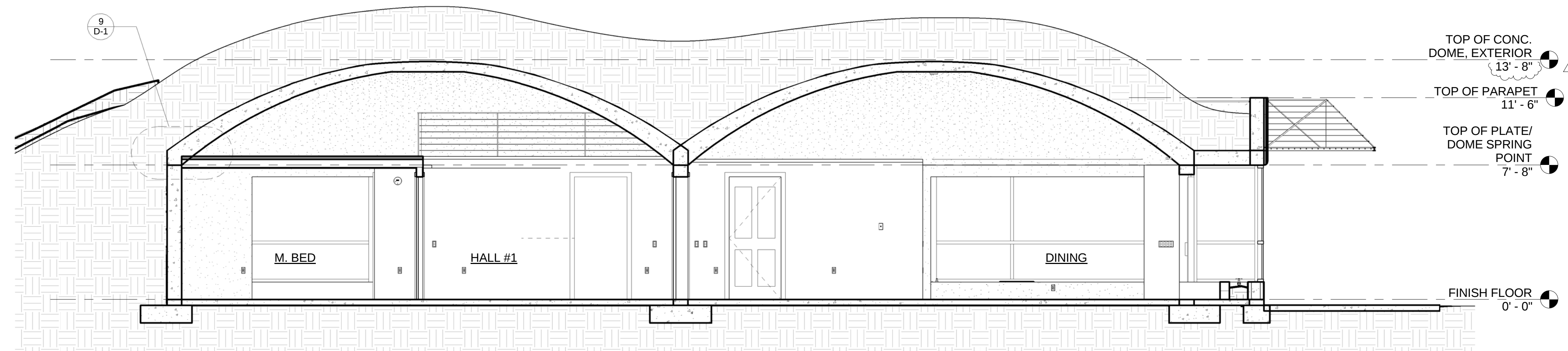
② CROSS SECTION 1 1/4" = 1'-0"
