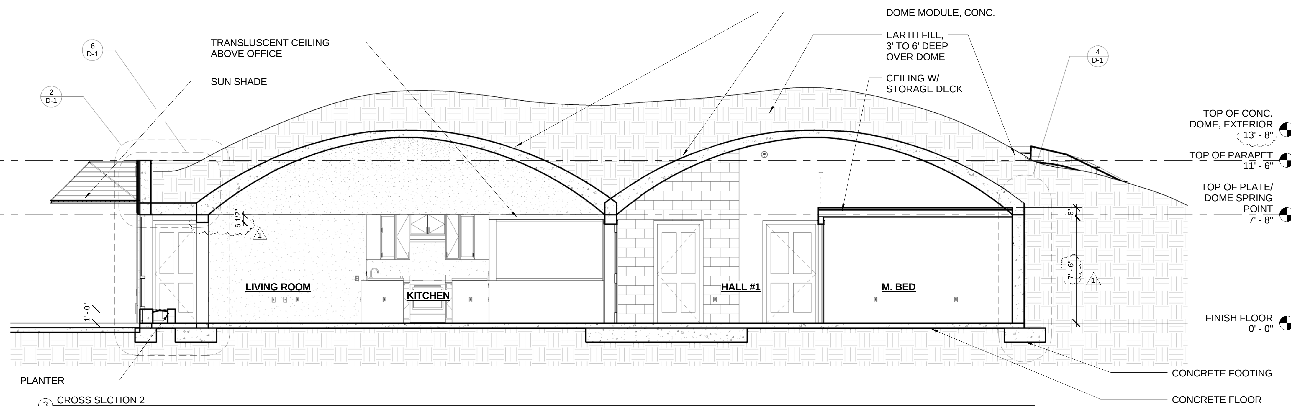
3 CROSS SECTION 2 1/4" = 1'-0"
