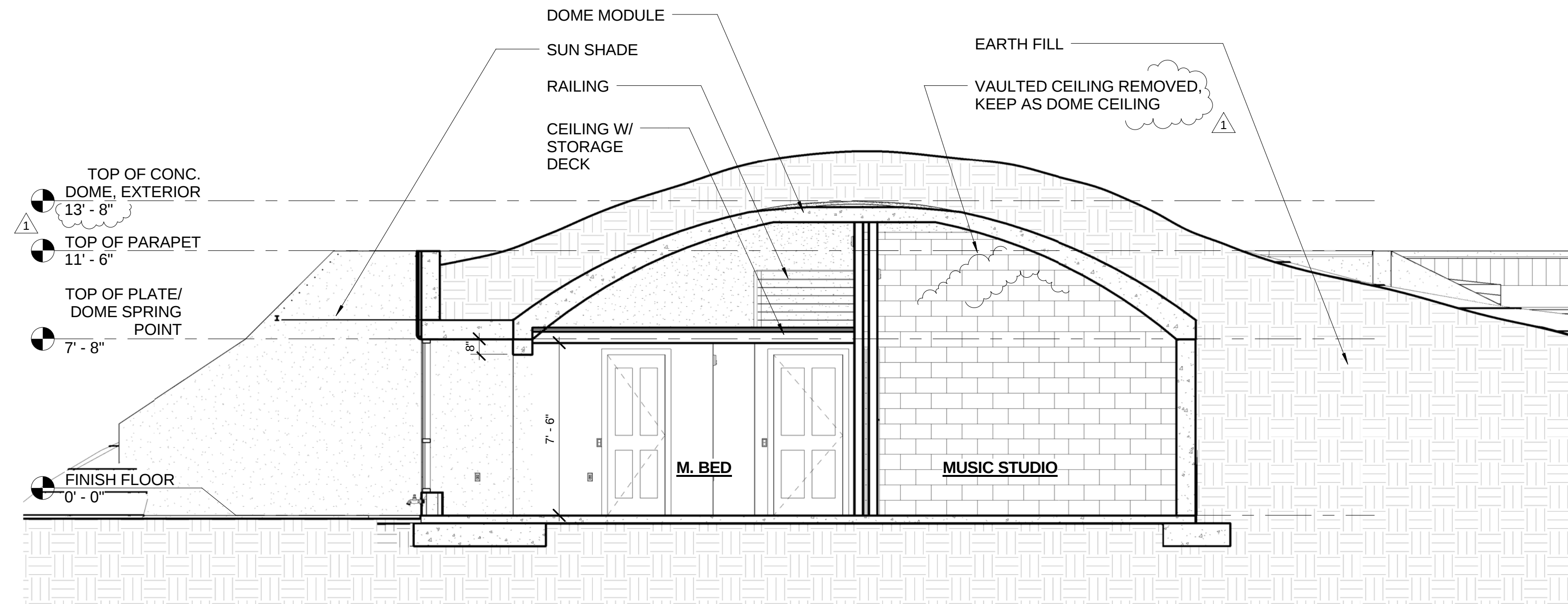
4 SECTION 4 1/4" = 1'-0"
